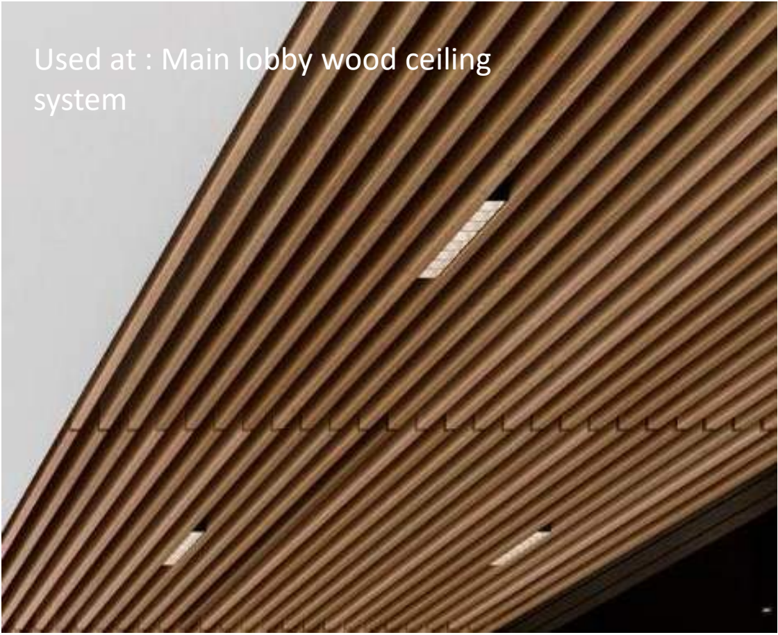
Armstrong Woodworks Grille 4" x 96" x 3/4" Red Oak on Poplar
